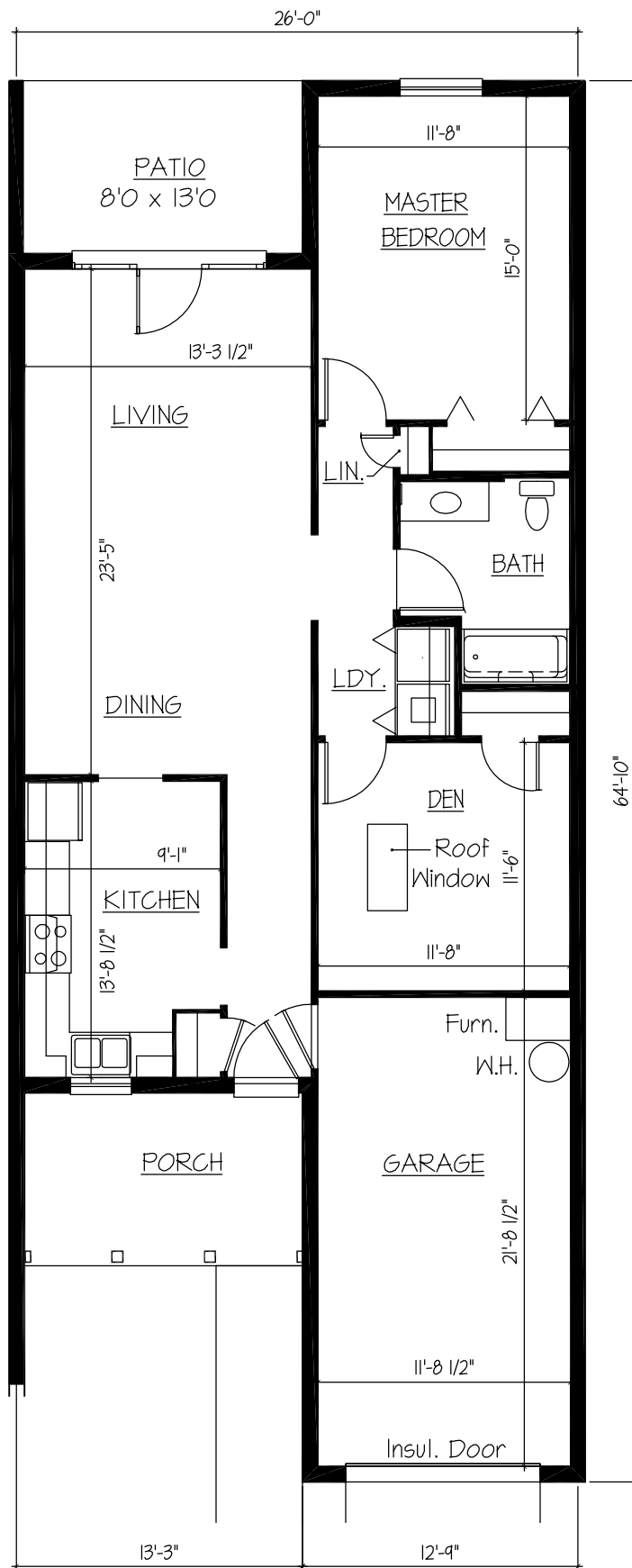
(A) FLOOR PLAN - 1/8" = 1'-0"
