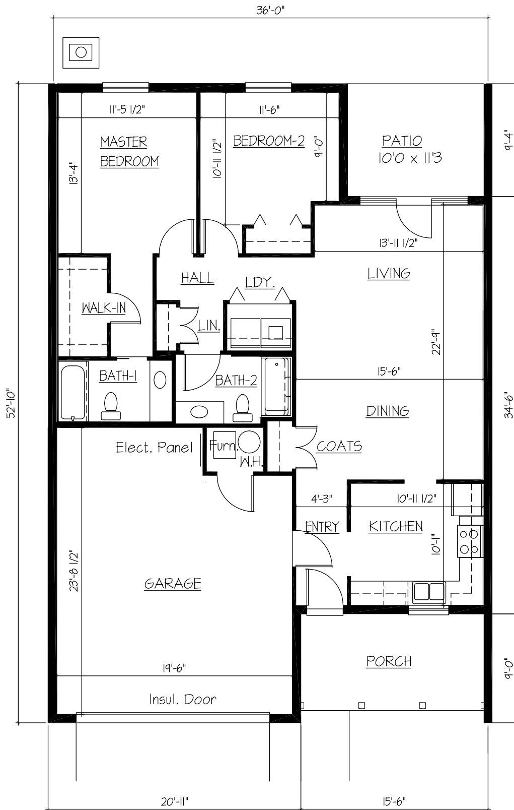
A FLOOR PLAN - 1/8" = 1'-0"
